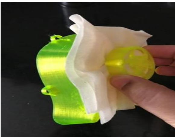
Photo: Prototypes of Face Shield, Flexible Face Mask without Filter and with Filter
