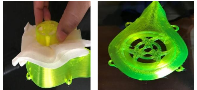
PLA Face Mask Design-3
