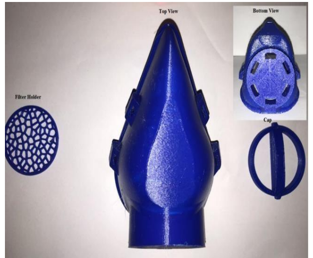
PLA Face Mask Design-2
